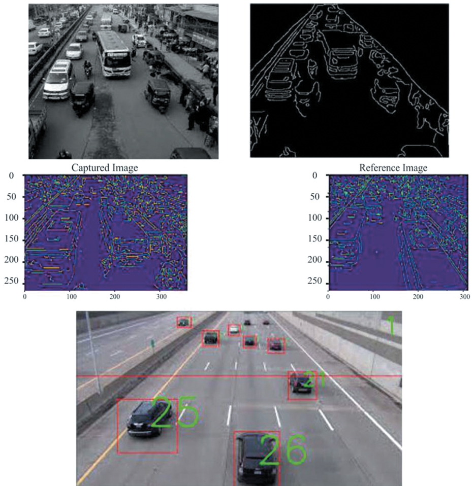
Figure 2.3: Image uploaded and click image processing using Canny edge detection.
